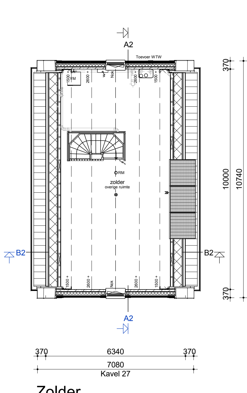
Zolder
