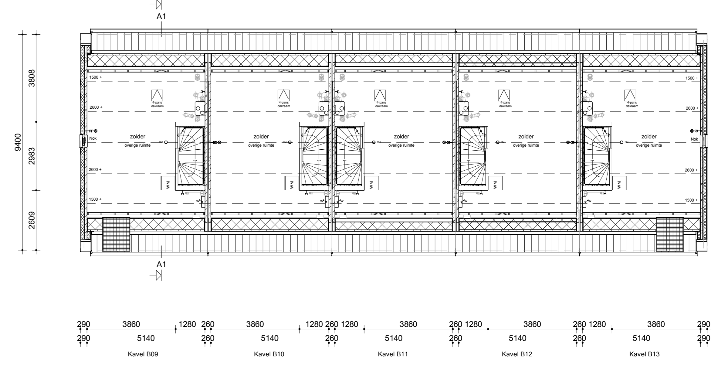
Zolder
