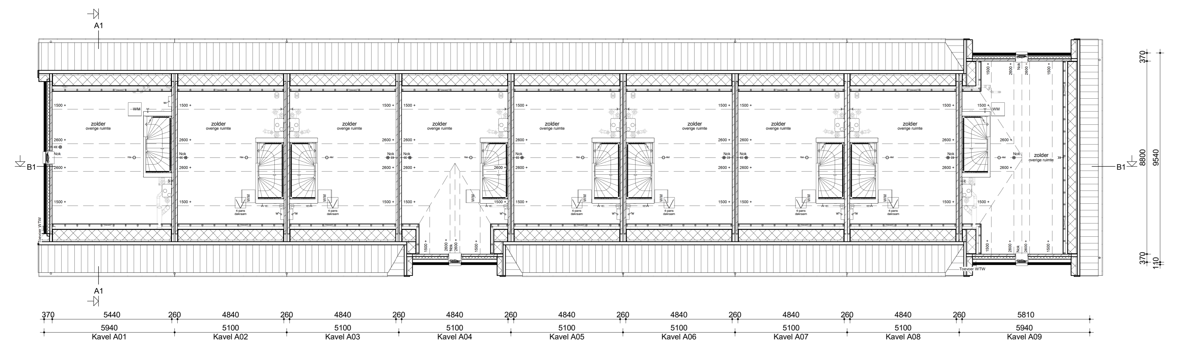
Zolder
