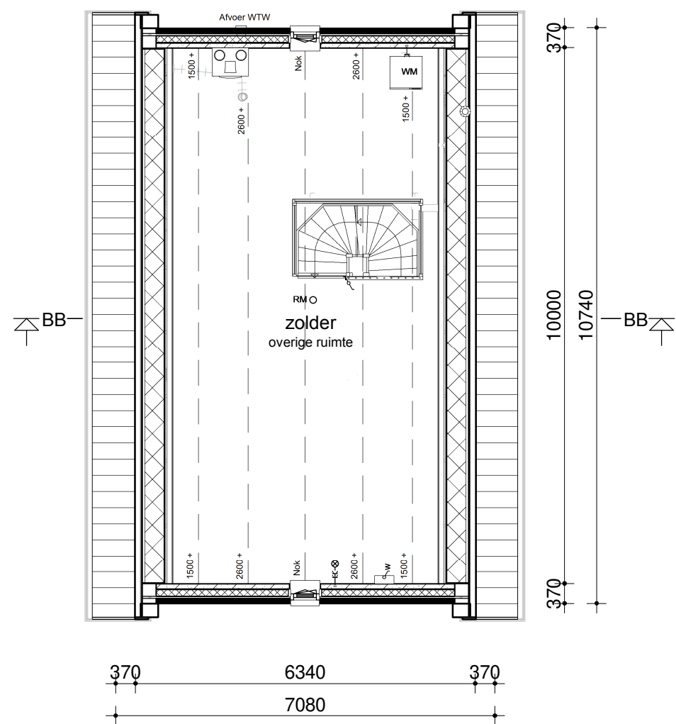
Zolder
