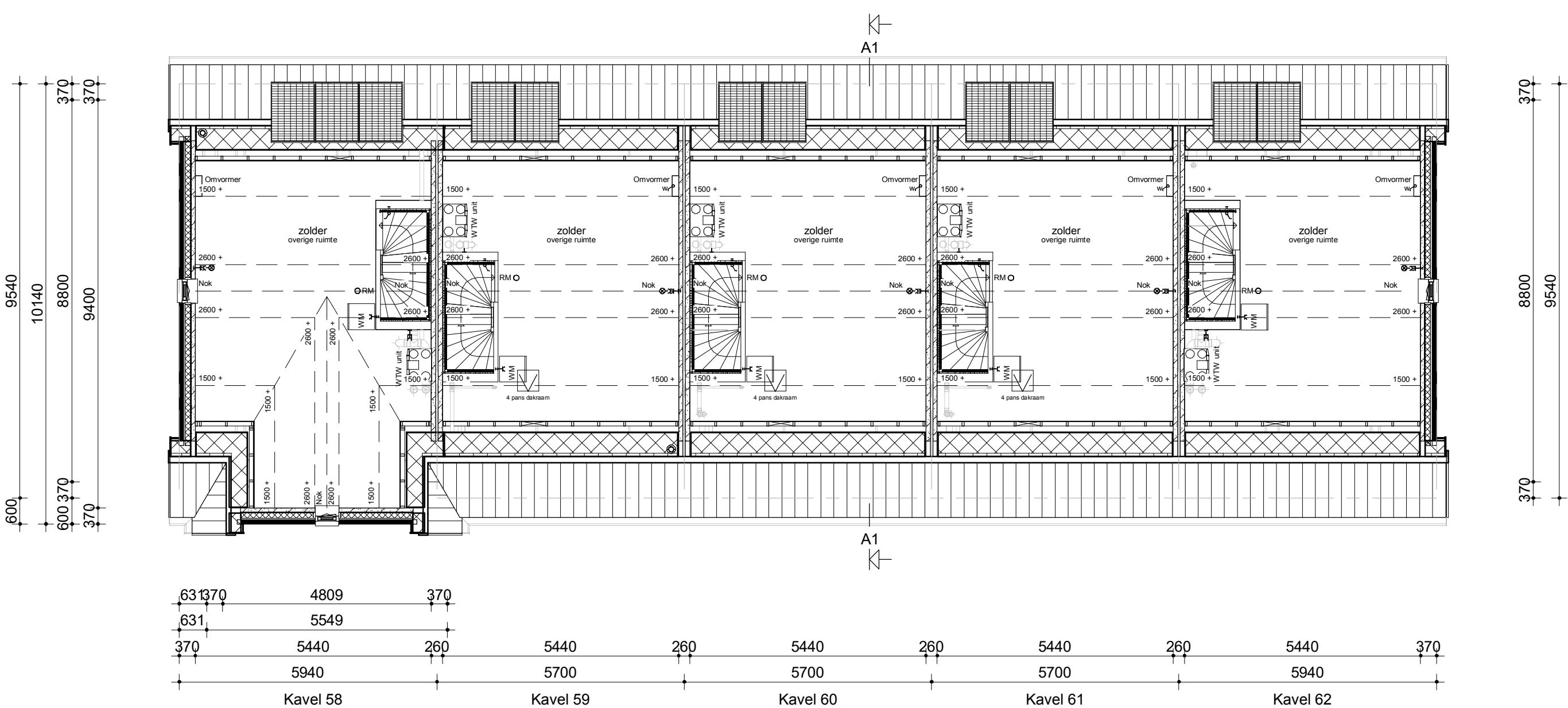
Zolder
