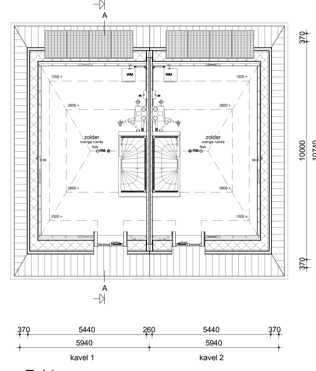
Zolder
