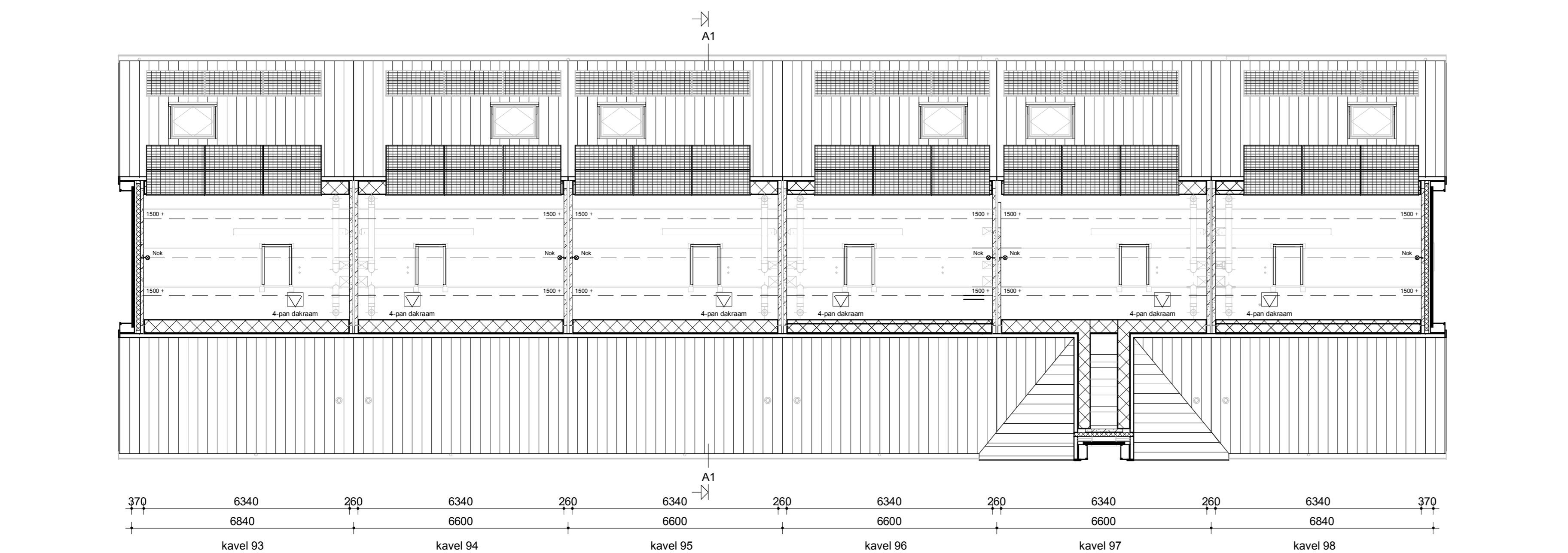
Zolder
