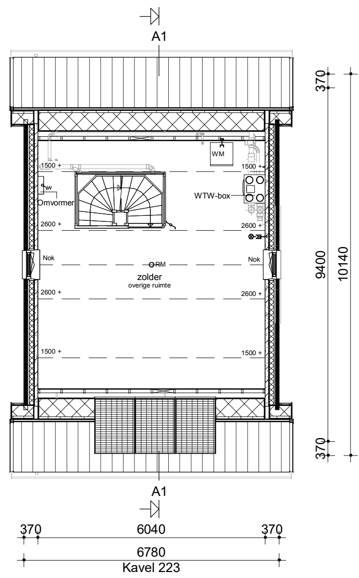
Zolder
