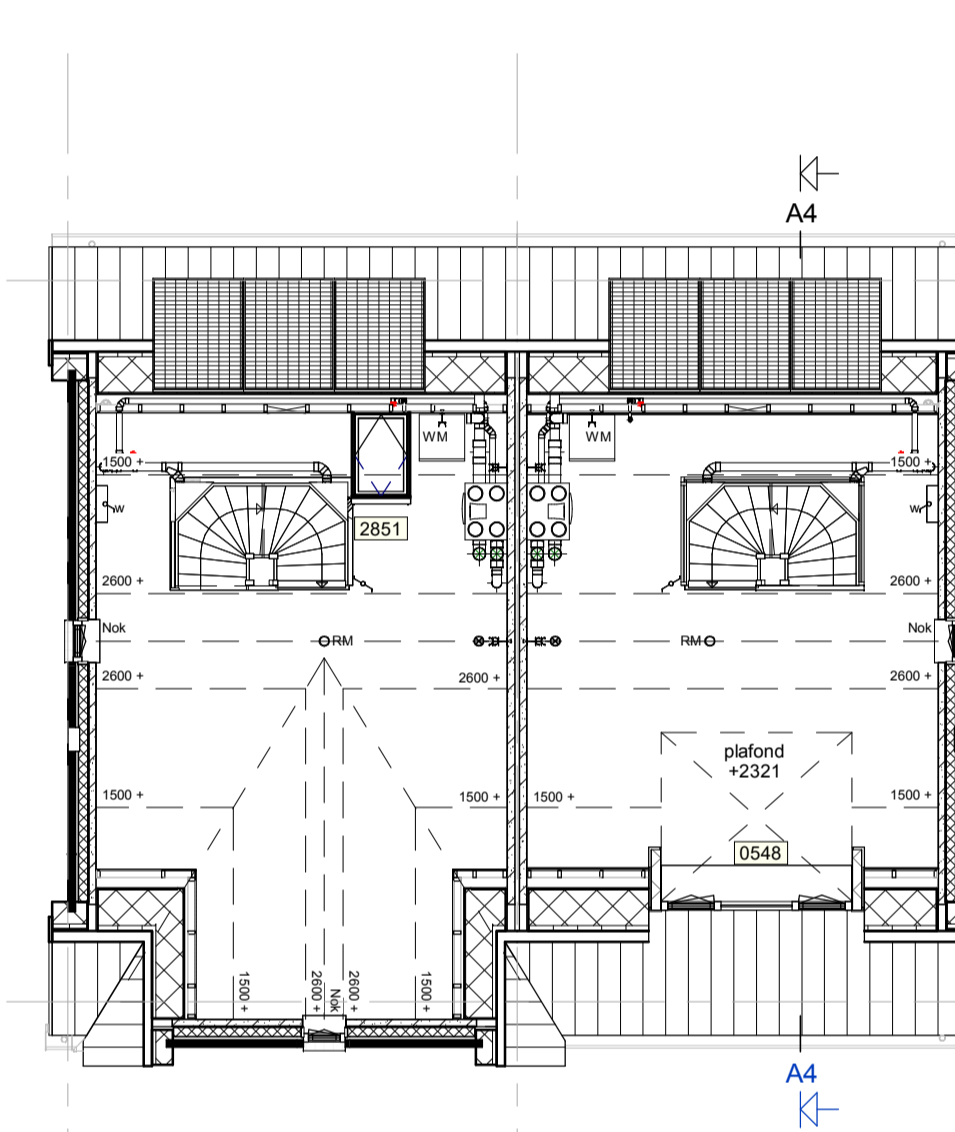
Zolder
