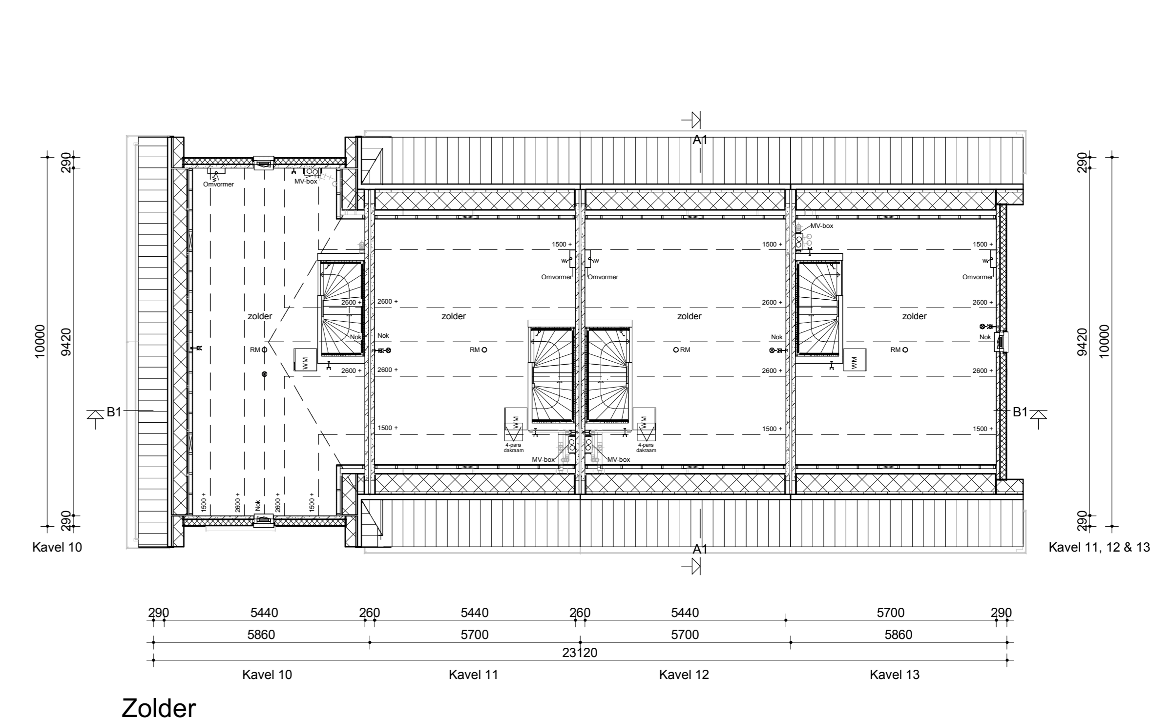
Zolder
