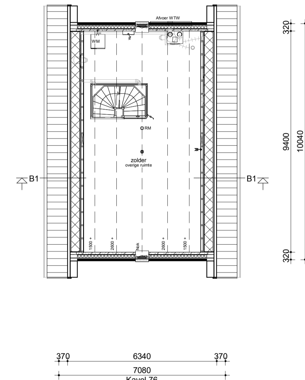
Zolder
