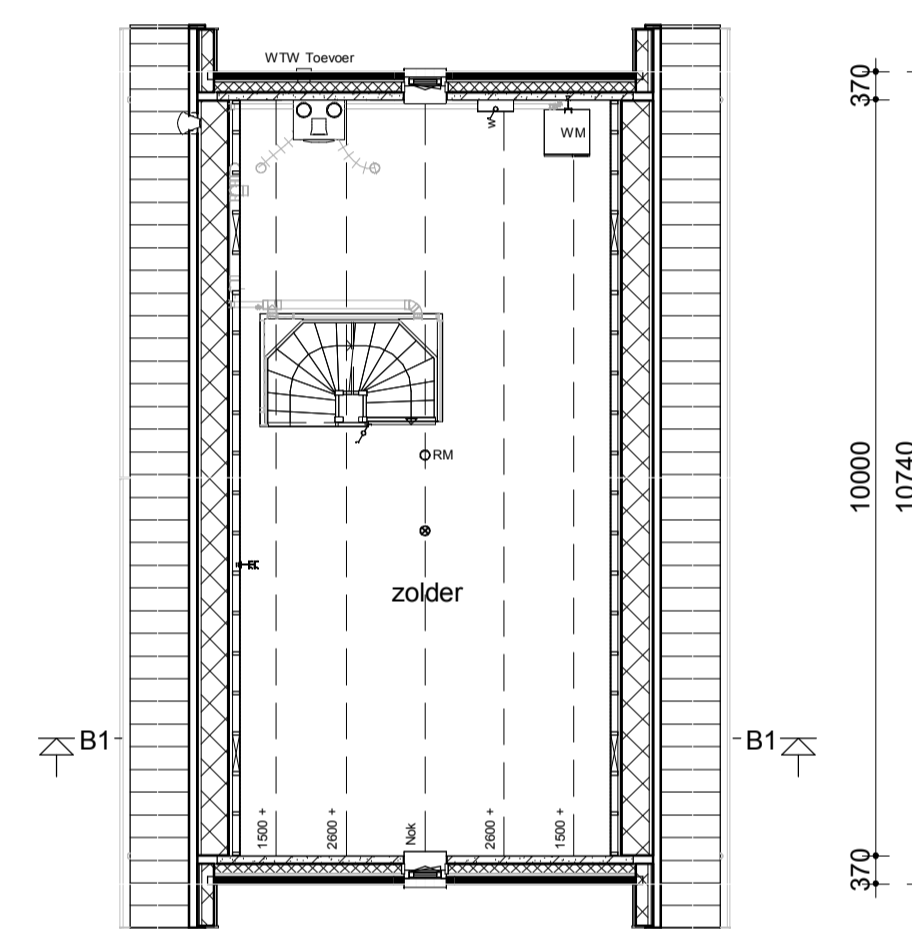
Zolder
