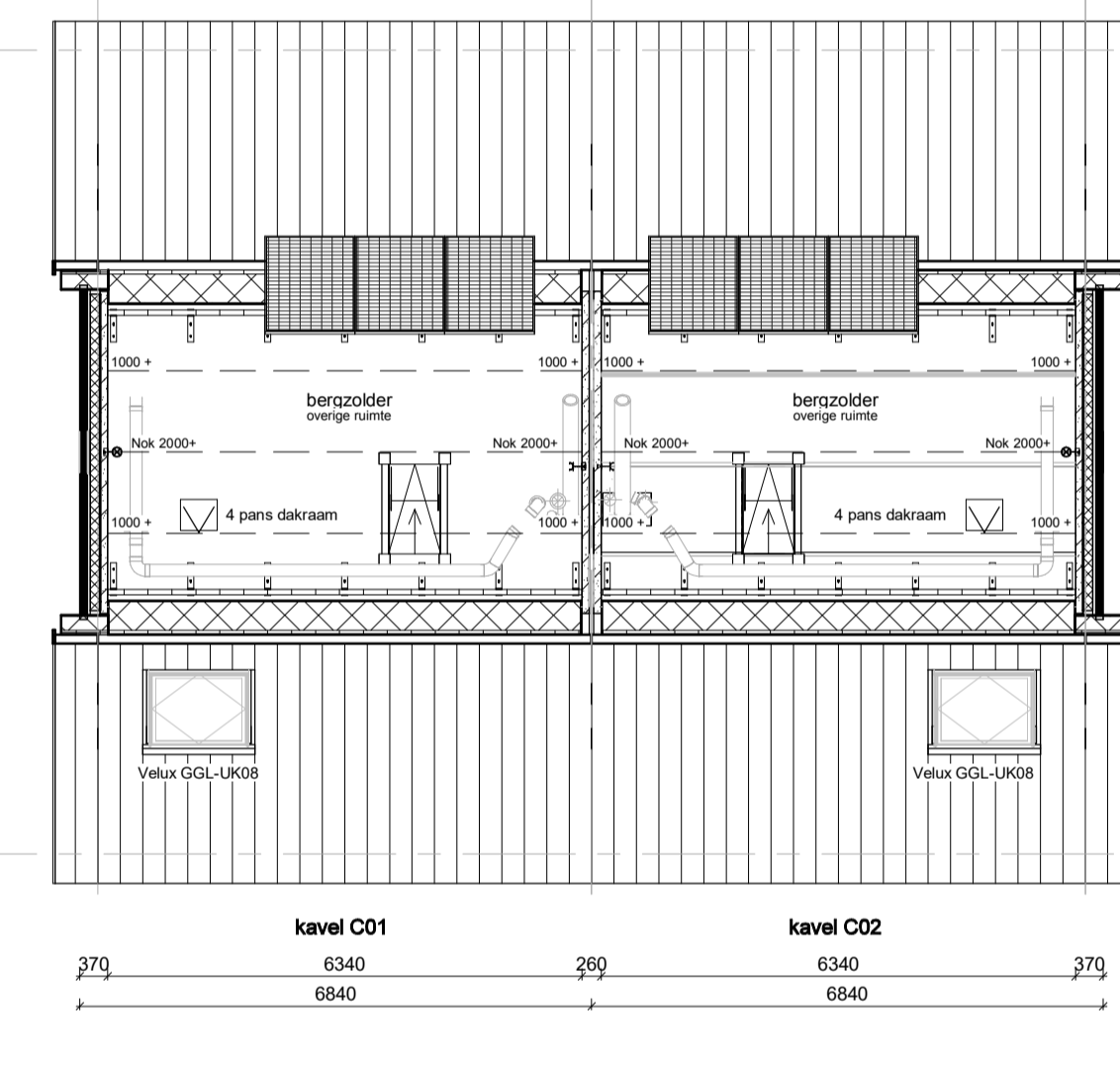
Zolder
