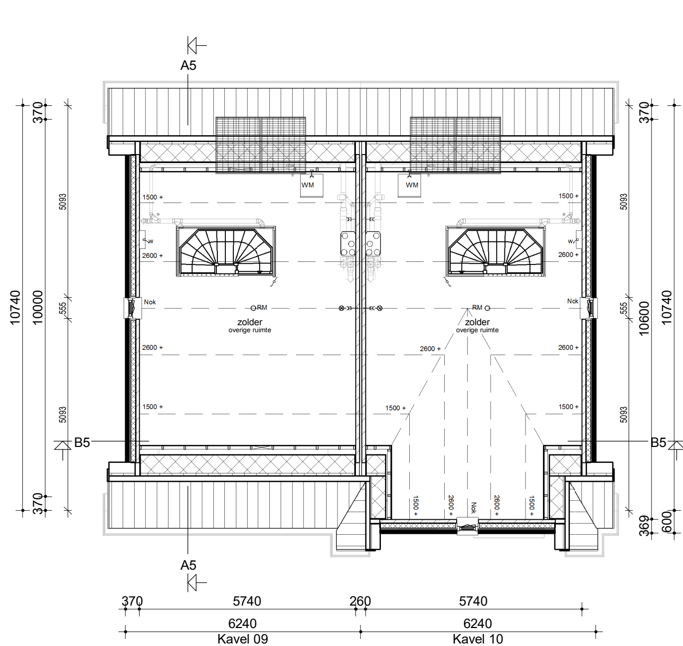
Zolder
