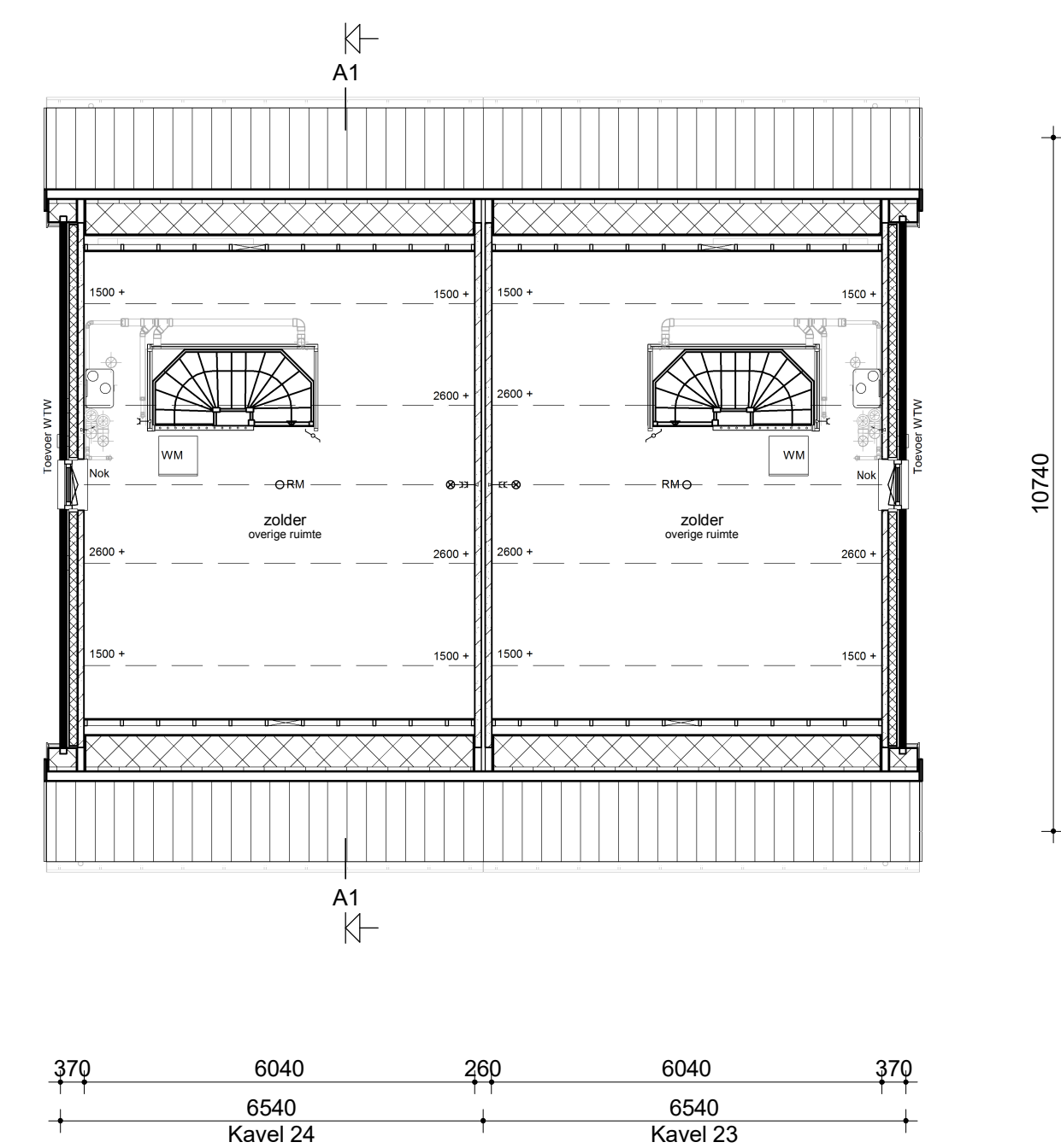
Zolder
