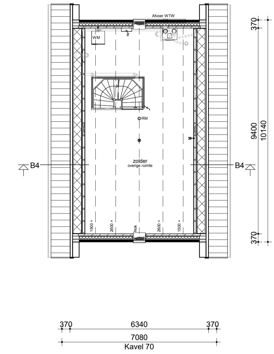
Zolder
